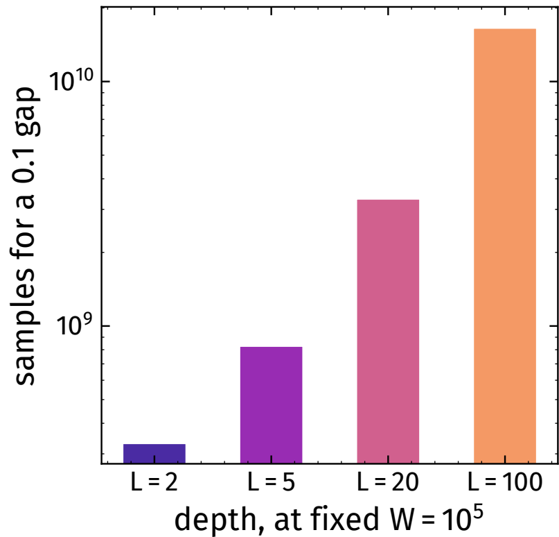
(b) the worst-case sample bound
