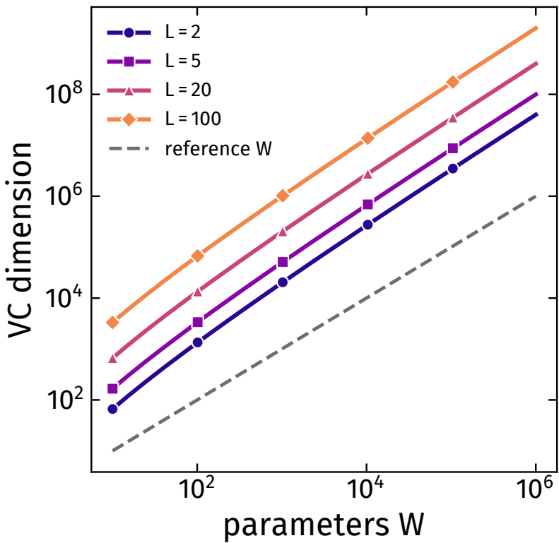
(a) \text{VCdim} = \Theta(WL\log W)
