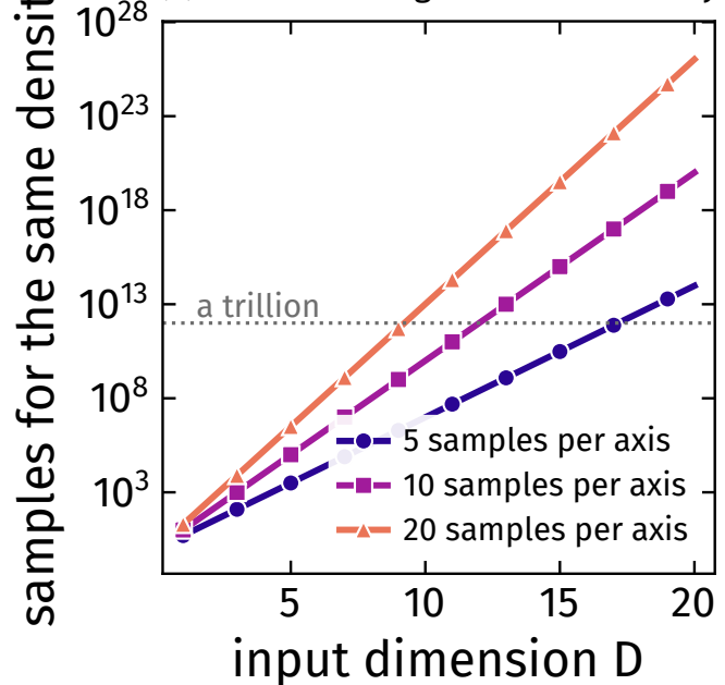
(c) data needed grows the same way
