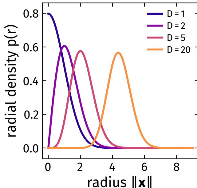
(b) Gaussian mass leaves the mode
