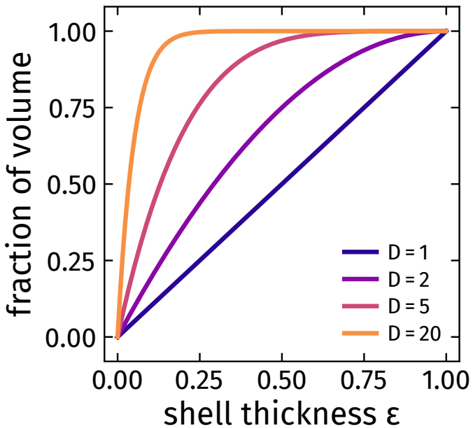
(a) 1 - (1 - \epsilon)^D : volume sits on the skin
