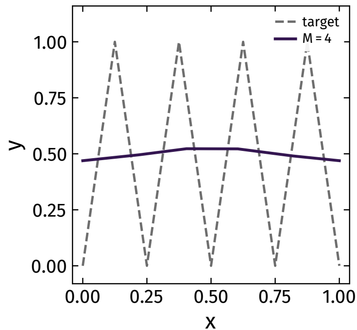
(a) shallow, M = 4 : \sup|f - \hat{y}| = 0.523
