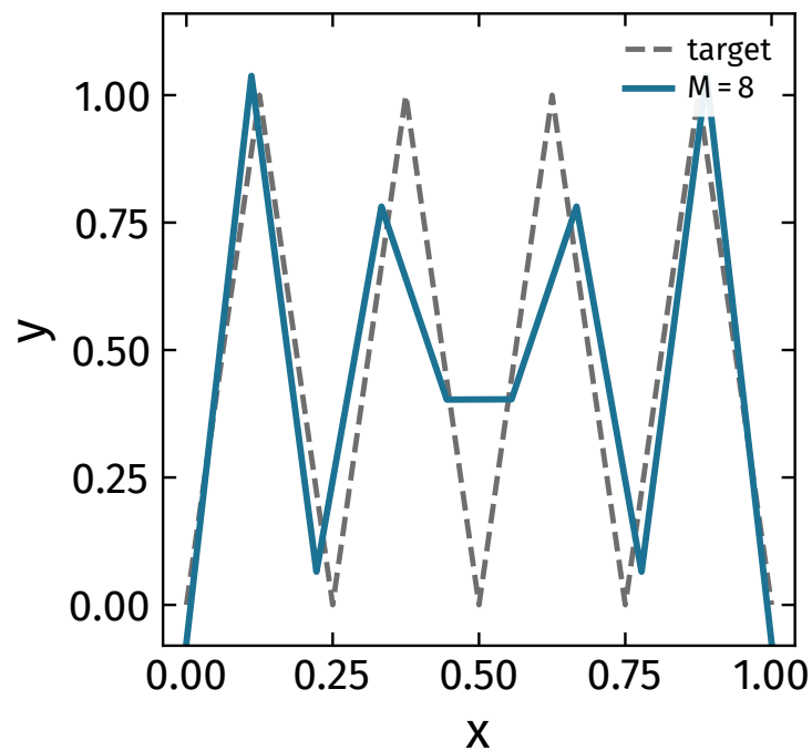
(b) shallow, M = 8 : \sup|f - \hat{y}| = 0.403
