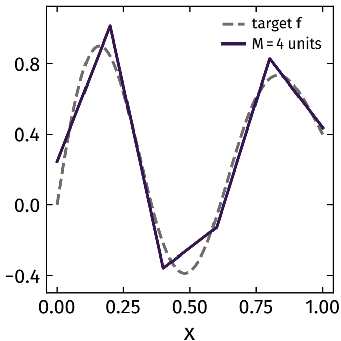
(a) M = 4 : \sup|f - \hat{y}| = 0.2446
