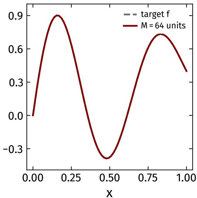
(c) M = 64 : \sup|f - \hat{y}| = 0.0015
