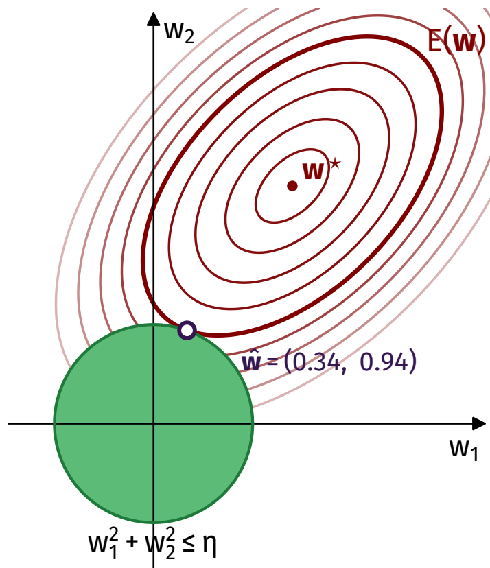
(b) q = 2 : weight decay
