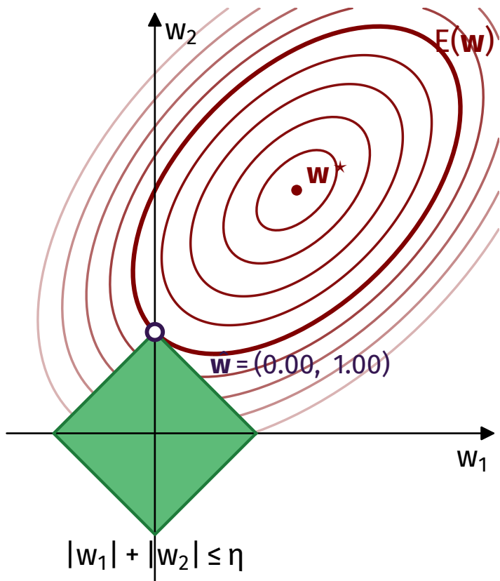
(a) q = 1 : the lasso
