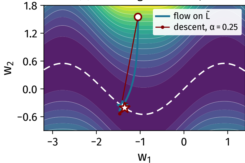
(c) loss + regularization, \tilde{L}
