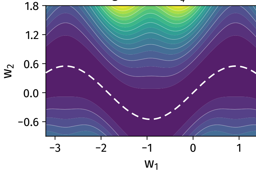
(b) regularization \frac{\alpha}{4} \|\nabla L\|^2
