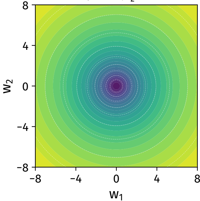
(b) penalty \frac{\lambda}{2} \|\mathbf{w}\|^2
