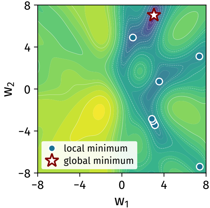
(a) loss E(\mathbf{w}) (9 minima)
