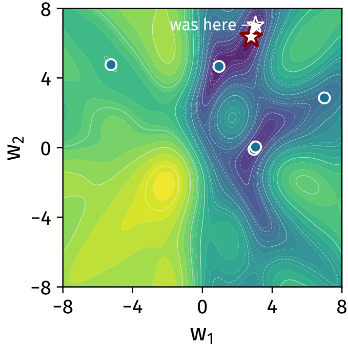
(c) loss + penalty (6 minima)
