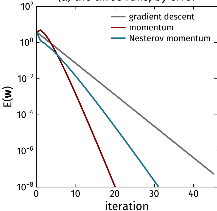
(a) the three runs, by error
