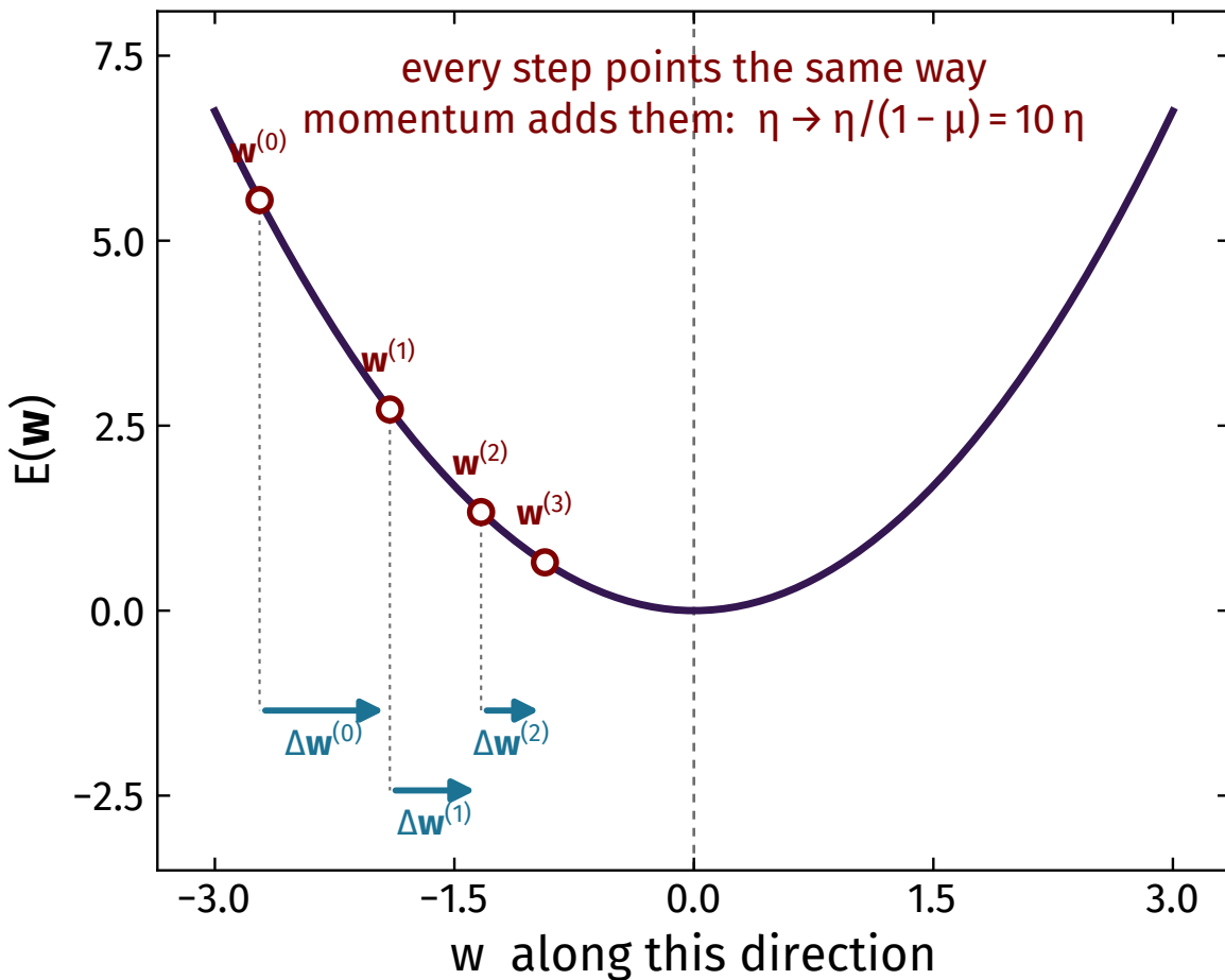
(a) low curvature: \eta\lambda = 0.30
