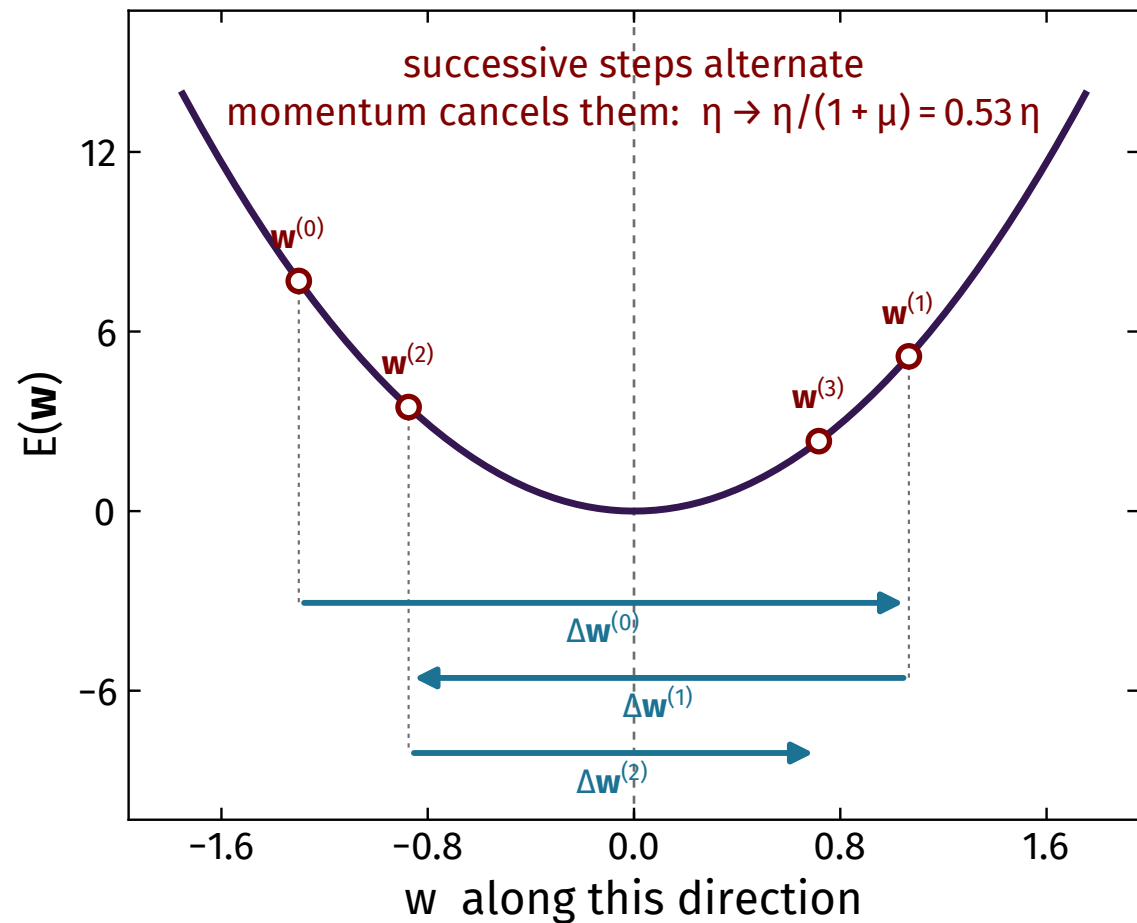
(b) high curvature: \eta\lambda = 1.82
