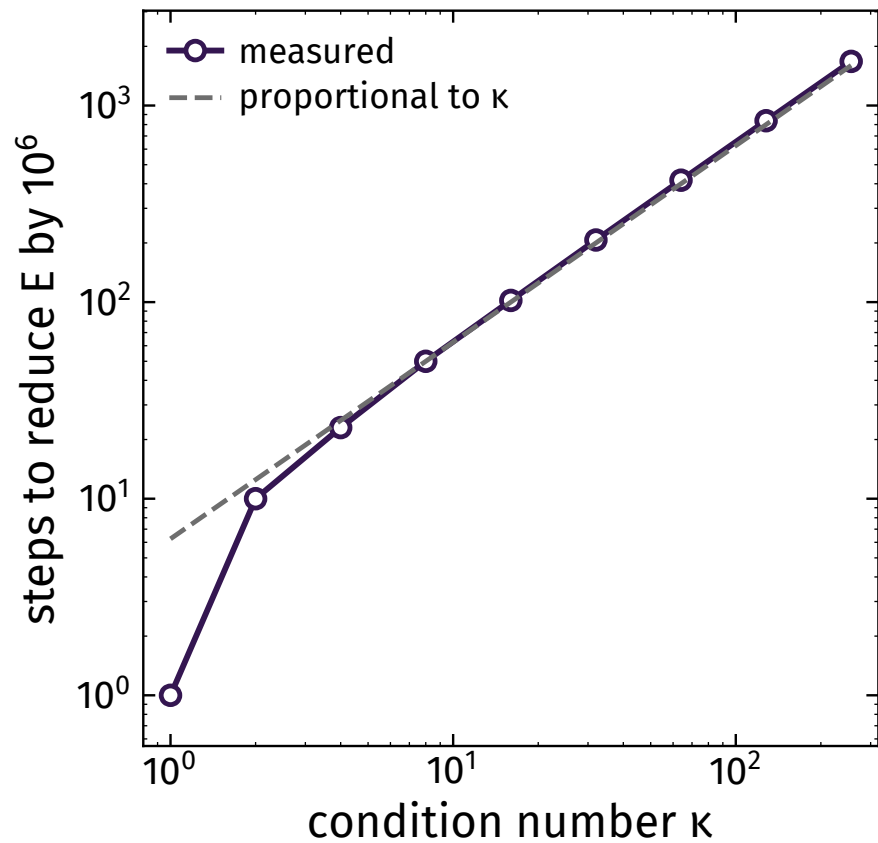
(b) the cost is linear in \kappa
