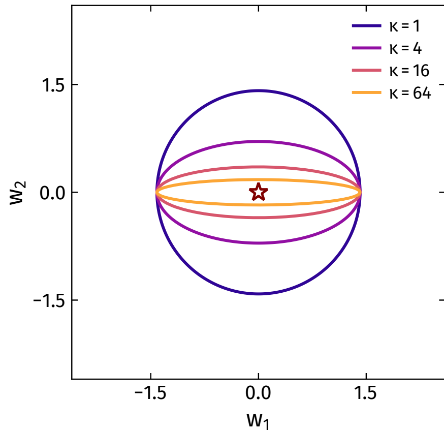
(a) one contour, four condition numbers
