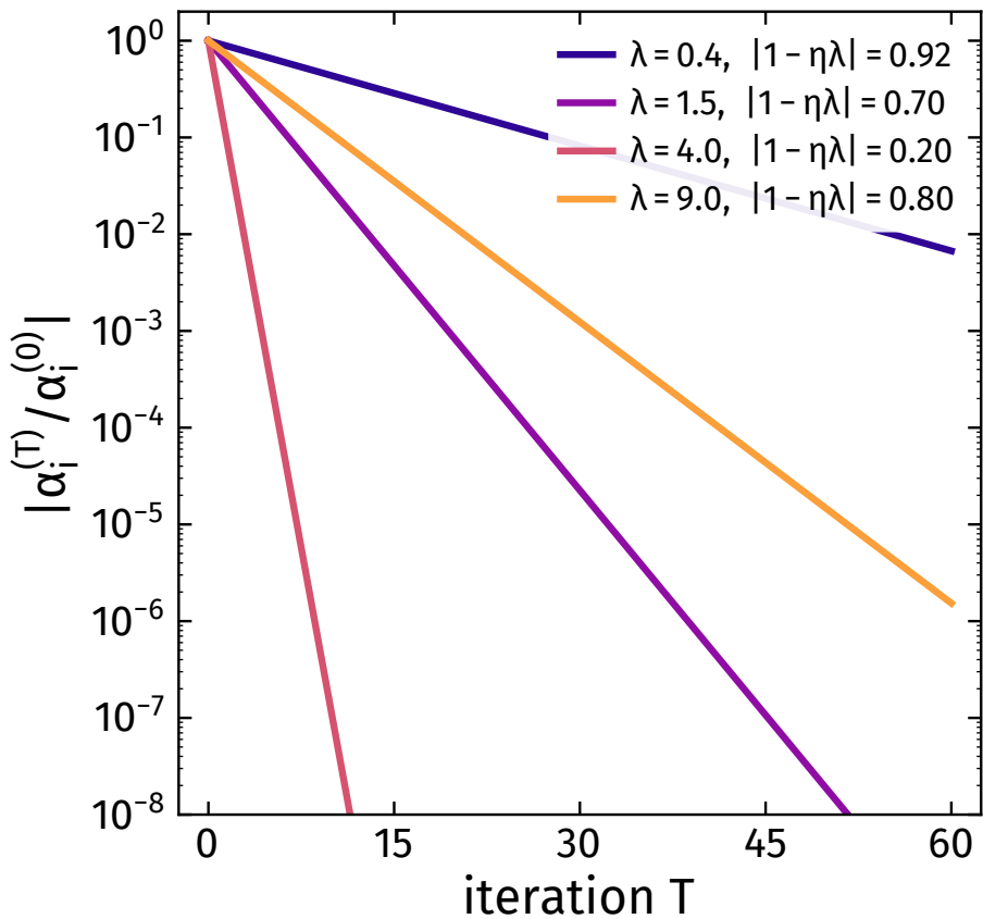
(a) one \eta = 0.20 , four curvatures
