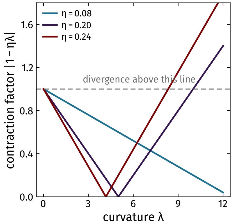
(b) stability needs \eta < 2/\lambda for every \lambda
