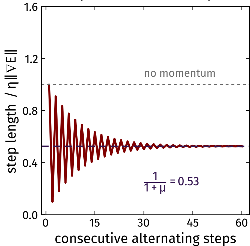
(b) alternating: the terms cancel (note the vertical scale)
