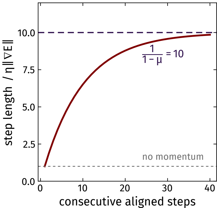
(a) aligned: \eta \rightarrow \eta/(1 - \mu)
