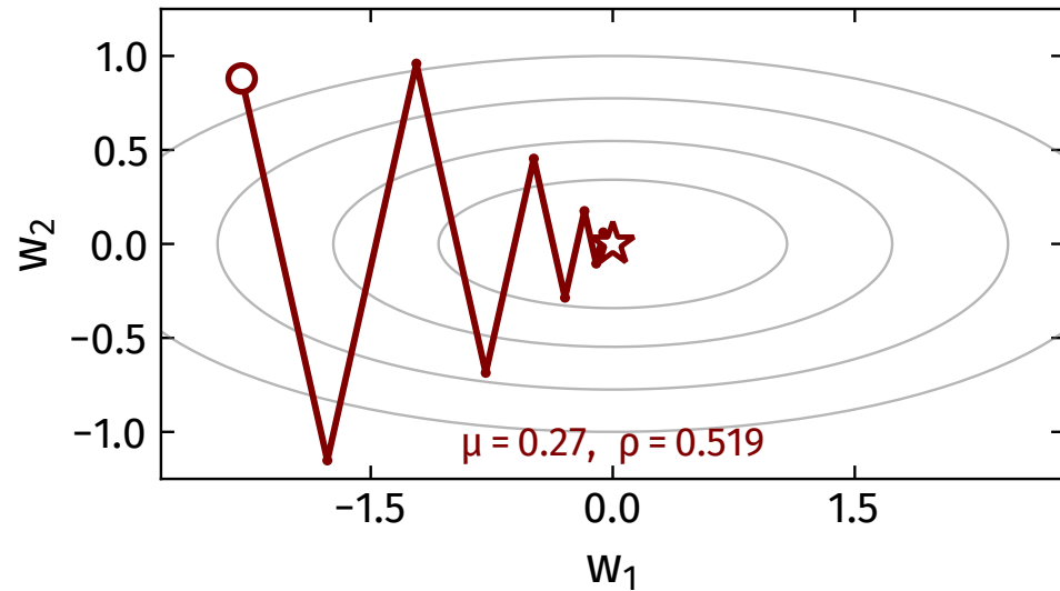
(b) momentum
