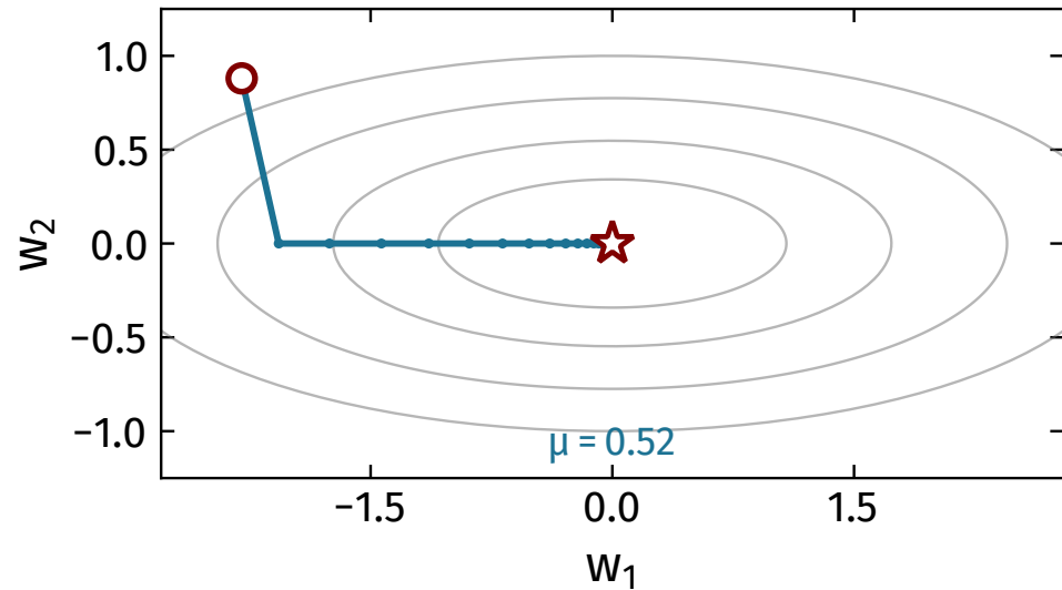
(c) Nesterov momentum
