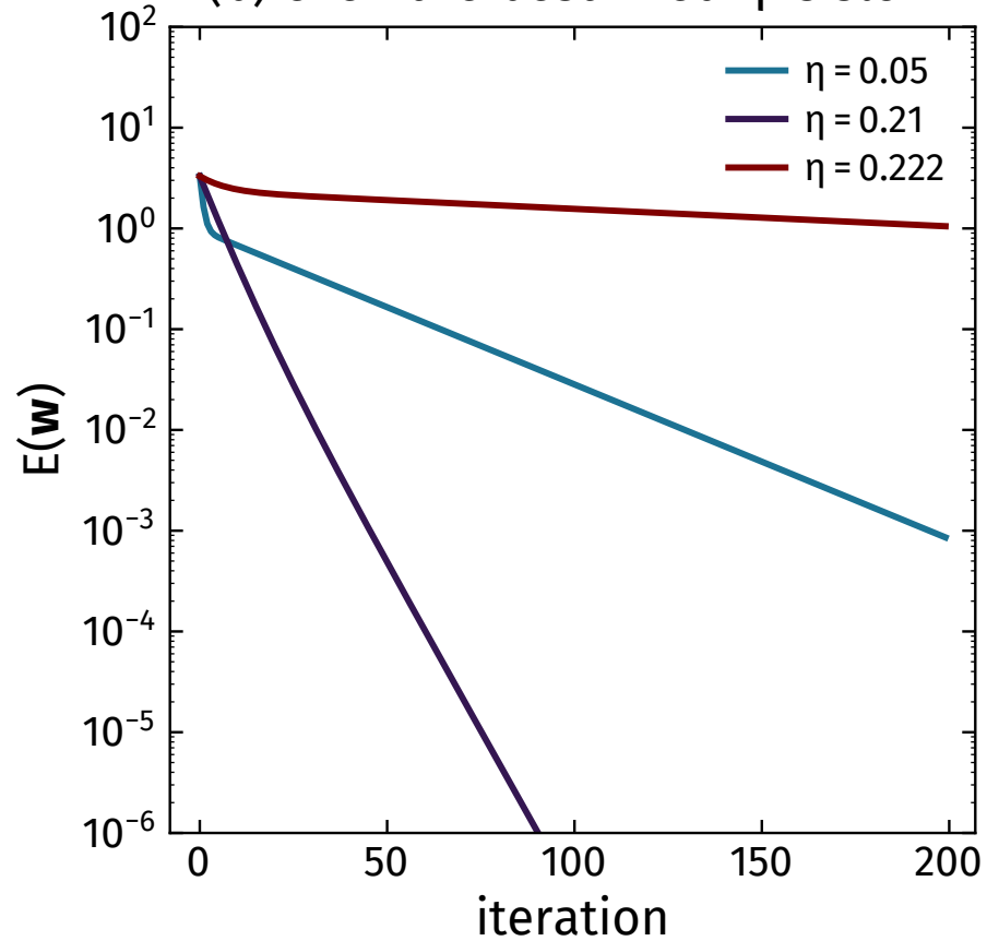
(b) even the best fixed \eta is slow
