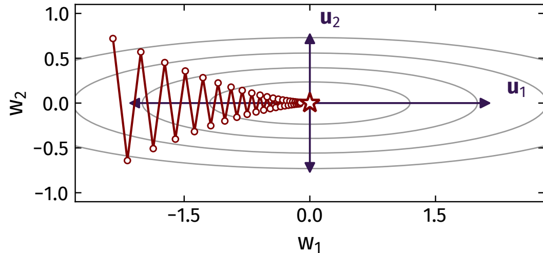
(a) \kappa = 26 : across fast, along slowly
