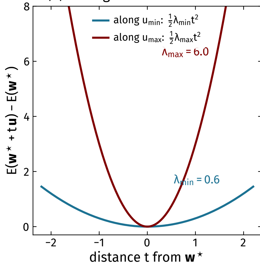
(b) the eigenvalue is a curvature
