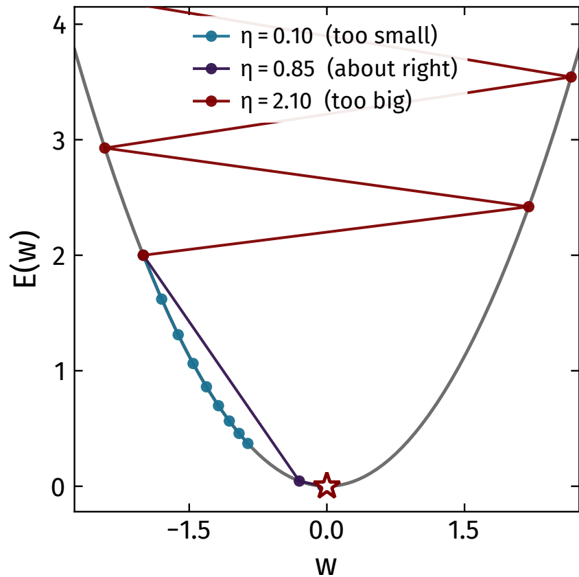
(b) the same three regimes, walked out
