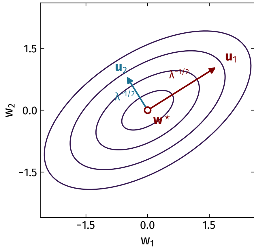
axes are the eigenvectors of H
