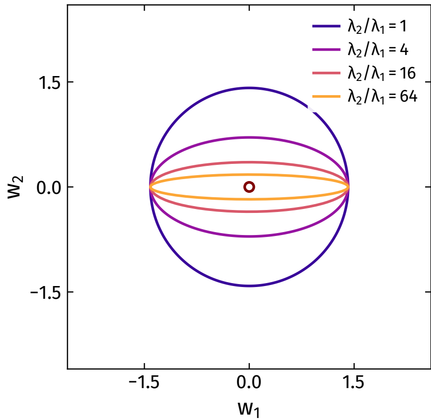
a wider spectrum is a narrower valley
