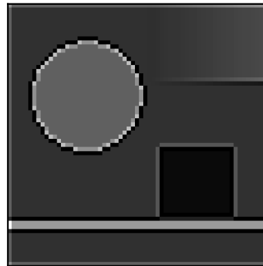
sharpen \alpha_4 = 0.027
