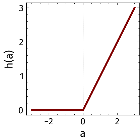
ReLU \max(0, a)
