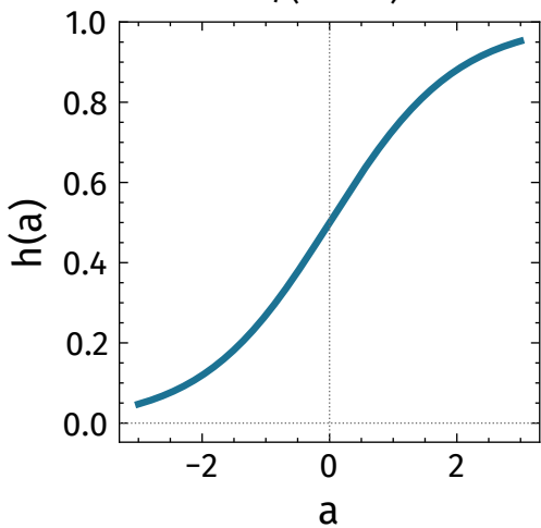
logistic sigmoid 1/(1 + e^{-a})
