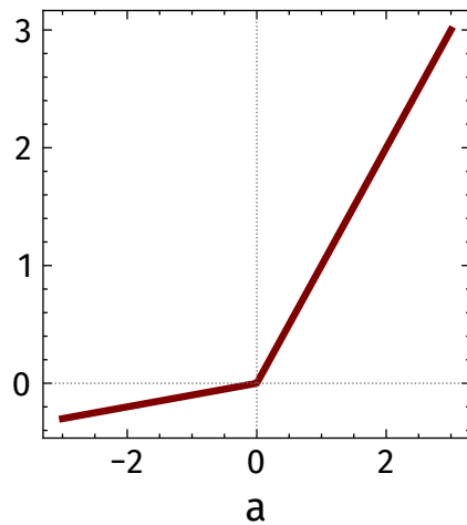
leaky ReLU \max(0.1a, a)
