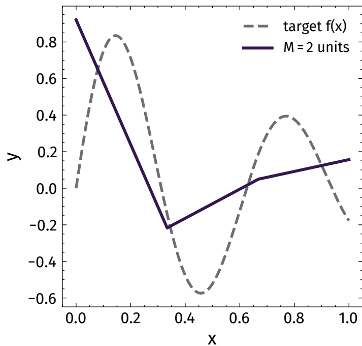
M=2 : M+1=3 linear pieces, \sup|f-\hat{y}| = 0.921
