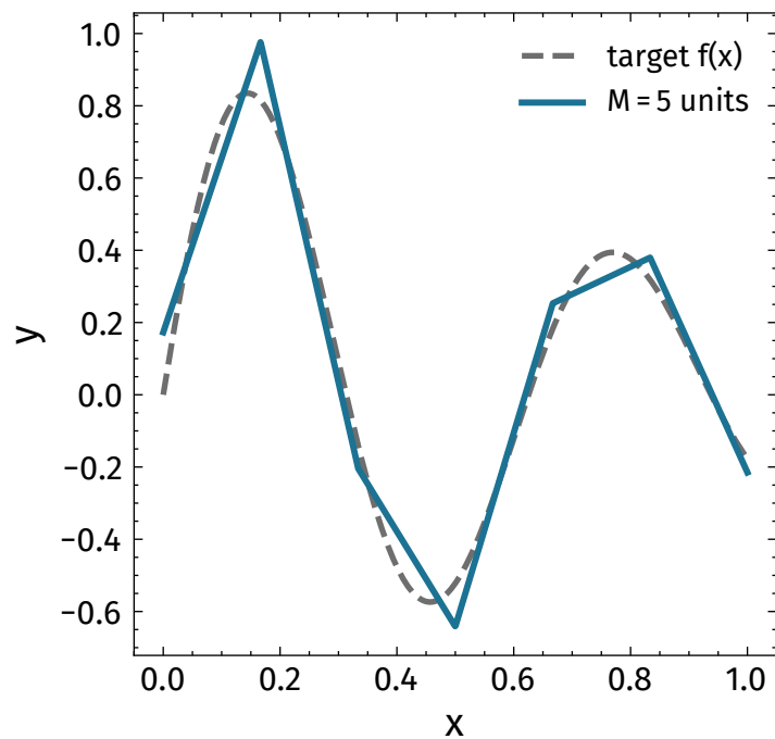
M=5 : M+1=6 linear pieces, \sup|f-\hat{y}| = 0.173
