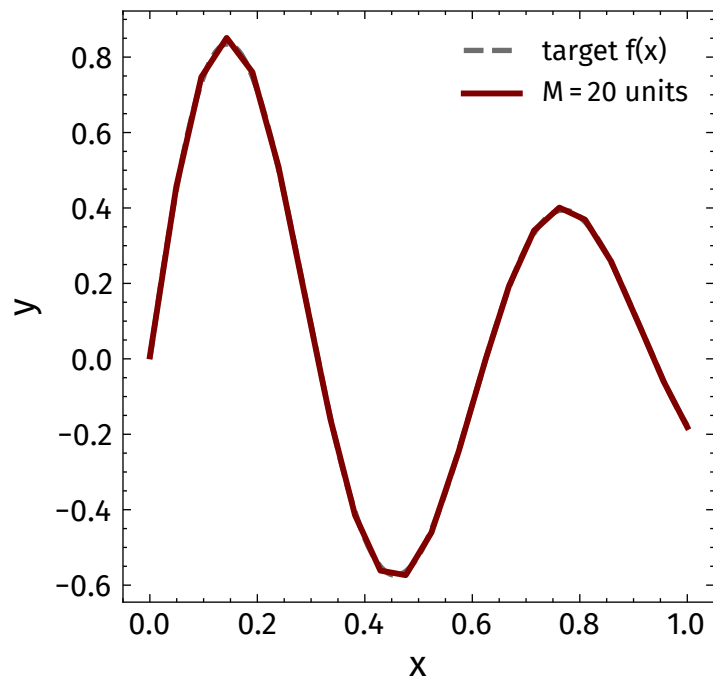
M=20 : M+1=21 linear pieces, \sup|f-\hat{y}| = 0.016
