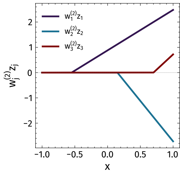
(d) each unit scaled by its output weight
