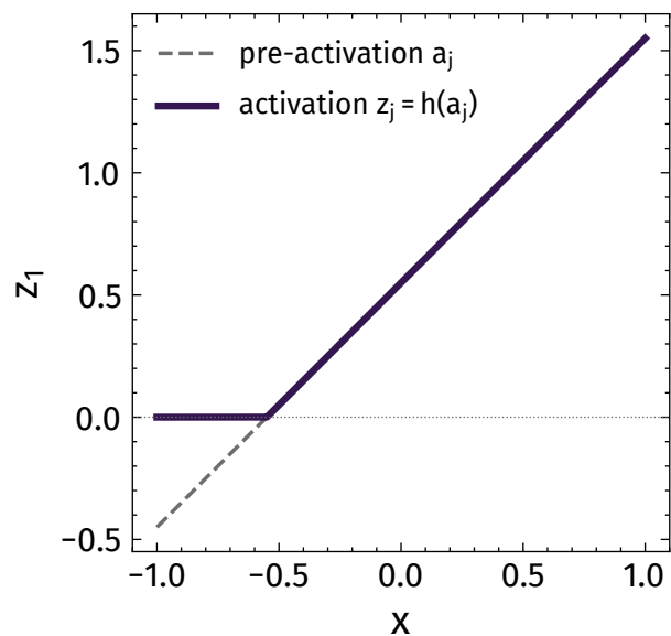
(a) z_1 = h(1x + 0.55)
