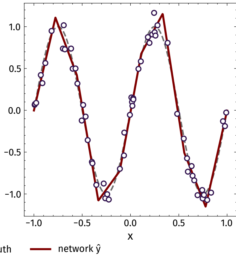
(b) f(x) = \sin(2\pi x) , M = 8 units
