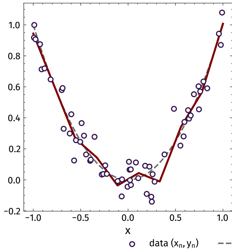
(a) f(x) = x^2 , M = 8 units
