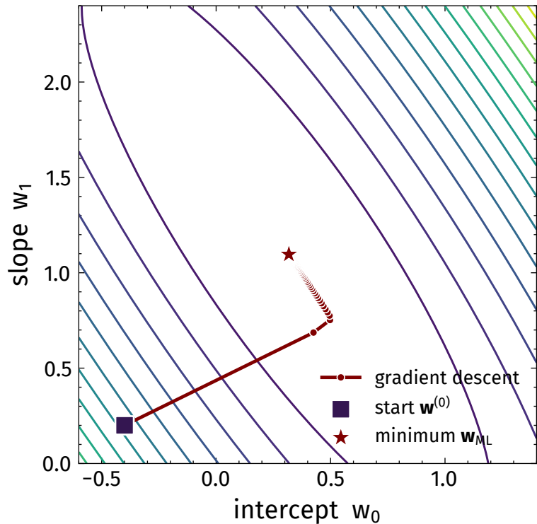
(b) one convex bowl, one minimum
