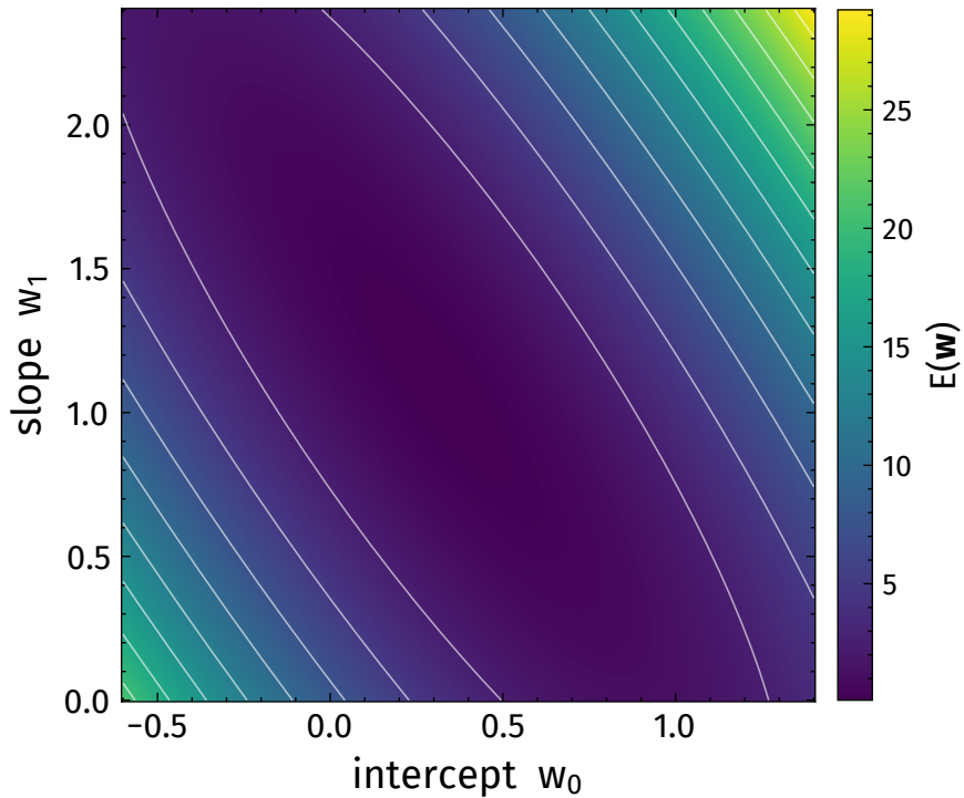
(a) the error surface E(\mathbf{w})
