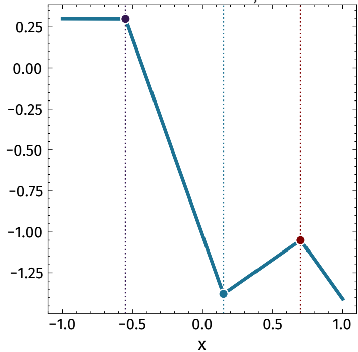
(b) output \hat{y}_2 = w_{20}^{(2)} + \sum_j w_{2j}^{(2)} z_j
