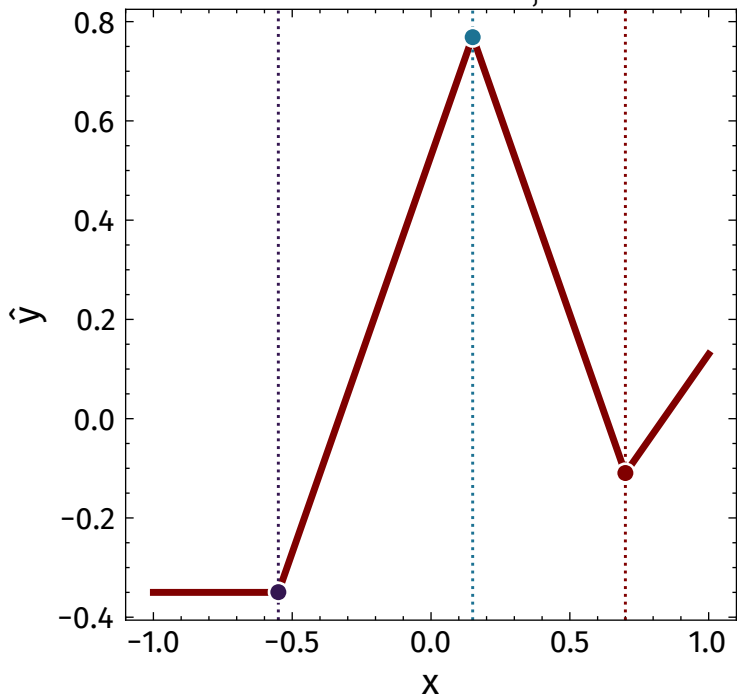
(a) output \hat{y}_1 = w_{10}^{(2)} + \sum_j w_{1j}^{(2)} z_j
