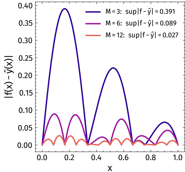
(c) \text{mesh} < \delta \Rightarrow \sup|f - \hat{y}| \leq \epsilon
