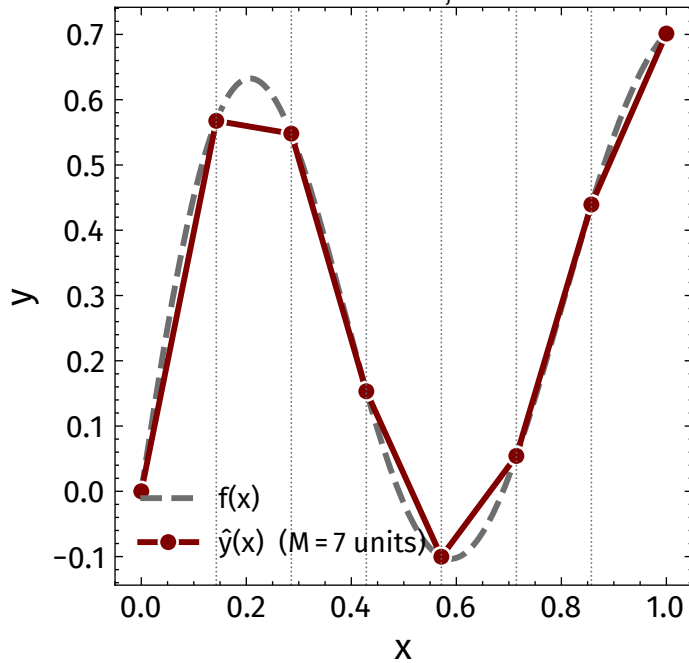
(b) \hat{y} = f(x_0) + s_1(x - x_0) + \sum_j (s_{j+1} - s_j)h(x - x_j)
