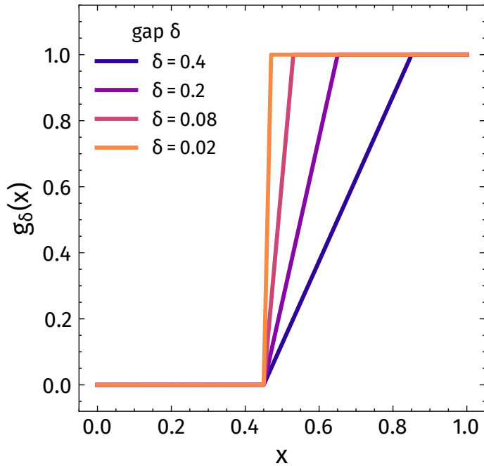
(a) \frac{1}{\delta}[h(x-a) - h(x-a-\delta)] \rightarrow \mathbb{1}[x > a]
