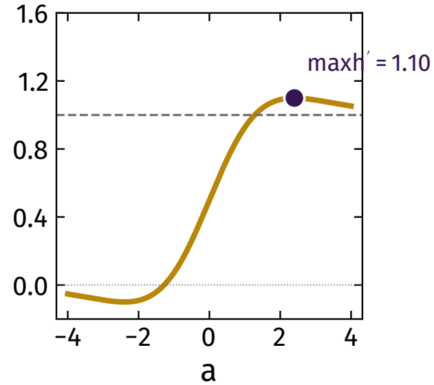
SiLU / swish
