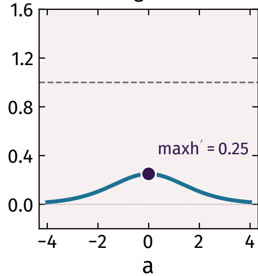
logistic
