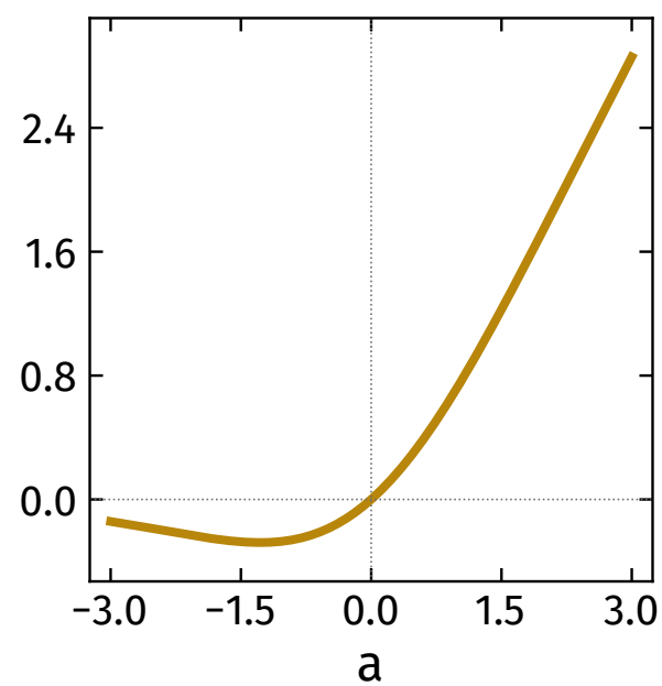
SiLU / swish a \sigma(a)
