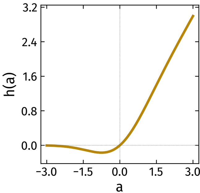
GELU a \Phi(a)
