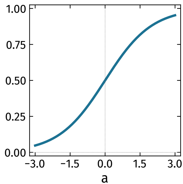
logistic 1/(1 + e^{-a})
