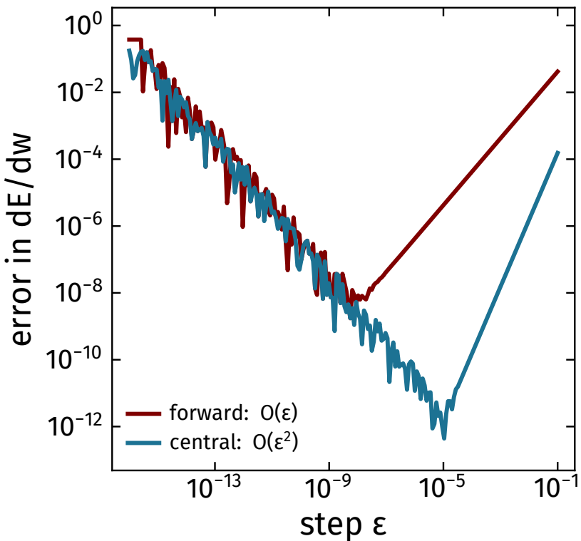
(a) truncation down, rounding up
