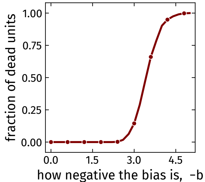
(c) a drifting bias switches units off for good
