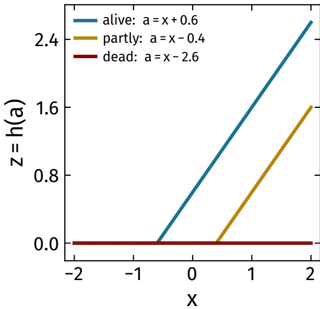
(a) three units over the data range
