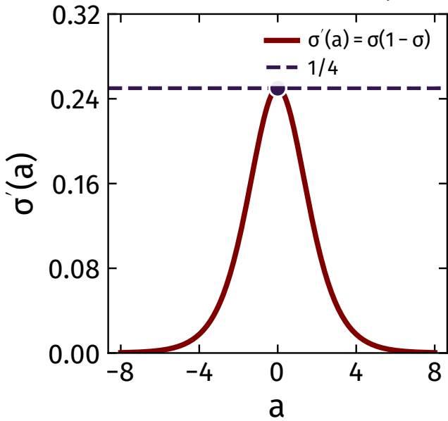
(a) the maximum is exactly 1/4
