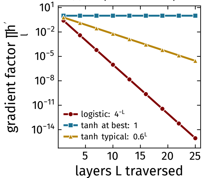
(c) the product over depth
