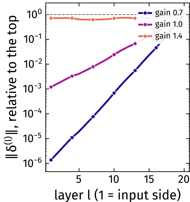
(b) ReLU
