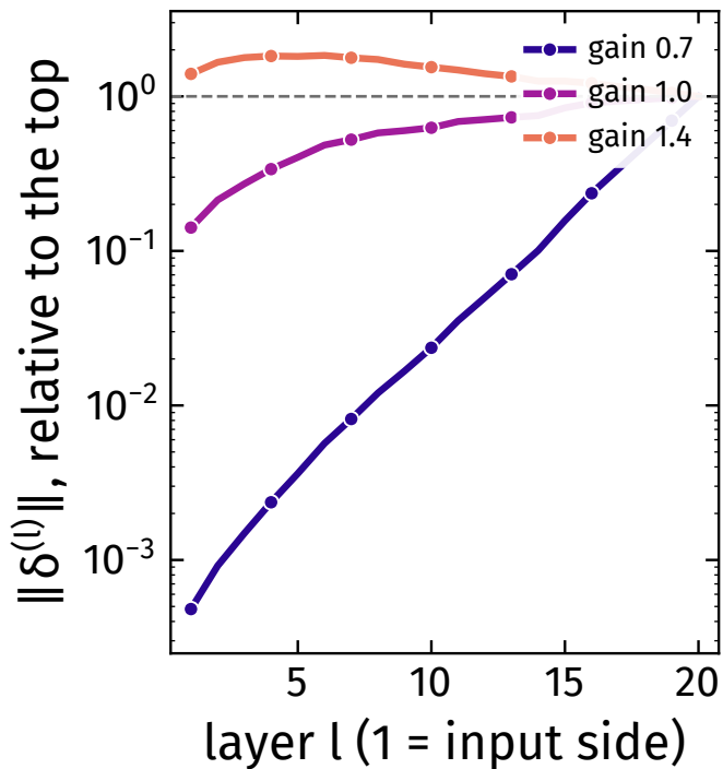
(a) tanh
