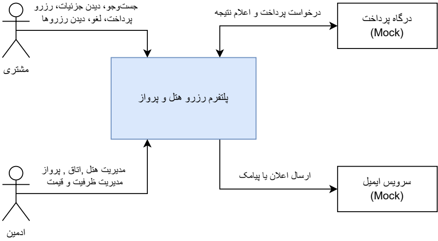
Context Diagram
