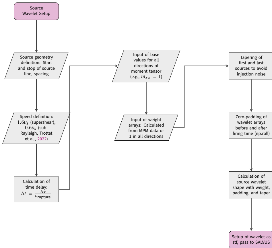
Figure 3.1: Operational workflow for the SALVUS source time function (STF) setup.
