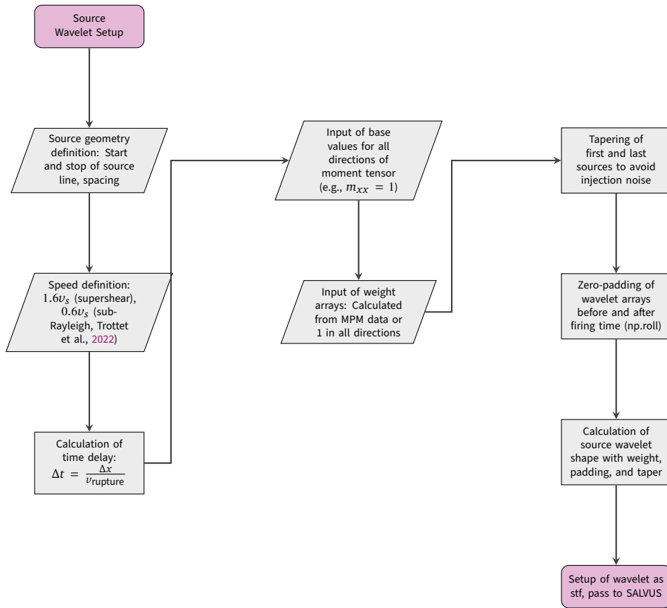
Figure 3.2: Operational workflow for the SALVUS source time function (STF) setup.
