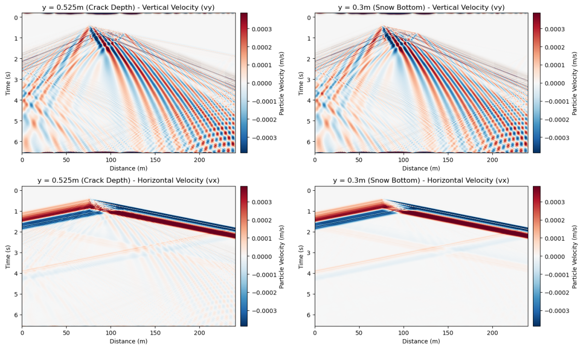
Figure 4.9: Particle velocity: vertical velocity in top row, horizontal velocity ( v_x ) in bottom row. Crack depth on left, snow bottom on the right. Colorbar shows magnitude of particle velocity (m/s).
