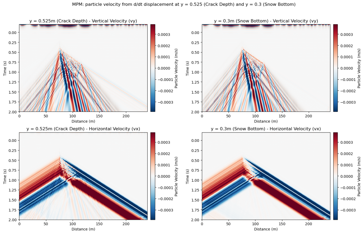
Figure 4.11: Particle velocity, zoomed into first arrival: vertical velocity in top row, horizontal velocity (vx) in bottom row. Crack depth on left, snow bottom on the right. Colorbar shows magnitude of particle velocity (m/s).
