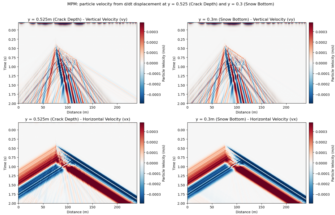
Figure 4.10: Particle velocity, zoomed into first arrival: vertical velocity in top row, horizontal velocity (vx) in bottom row. Crack depth on left, snow bottom on the right. Colorbar shows magnitude of particle velocity (m/s).
