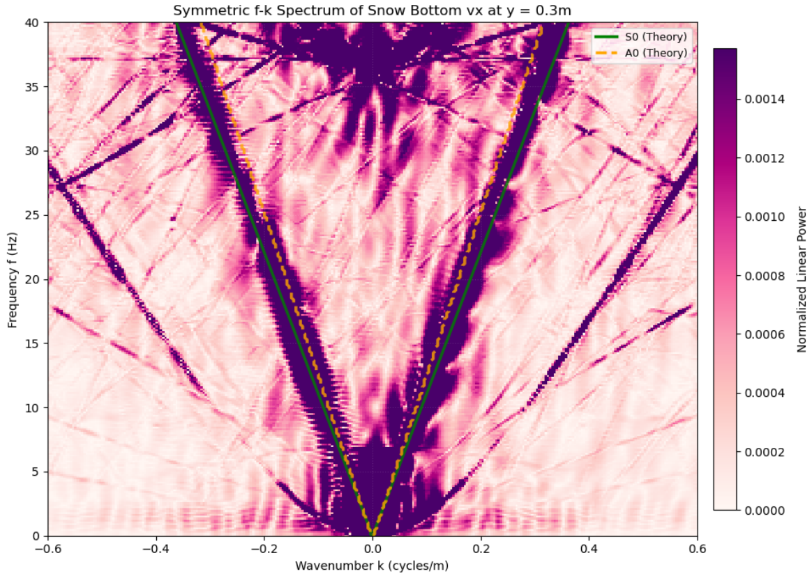
Figure 4.13: F-k plot for the MPM-guided simulation. Lamb wave dispersion curves calculated from ???. A0 mode shown in orange, S0 mode in green. Colorbar shows energy normalized to the 99th percentile.
