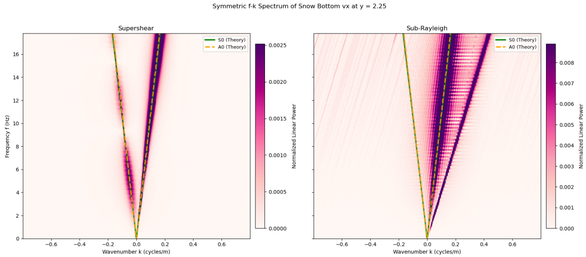
Figure 4.6: F-k plot for the Supershear (left) and sub-Rayleigh (right) case. Lamb wave dispersion curves calculated from ???. A0 mode shown in orange, S0 mode in green. Colorbar shows energy normalized to the 99th percentile.
