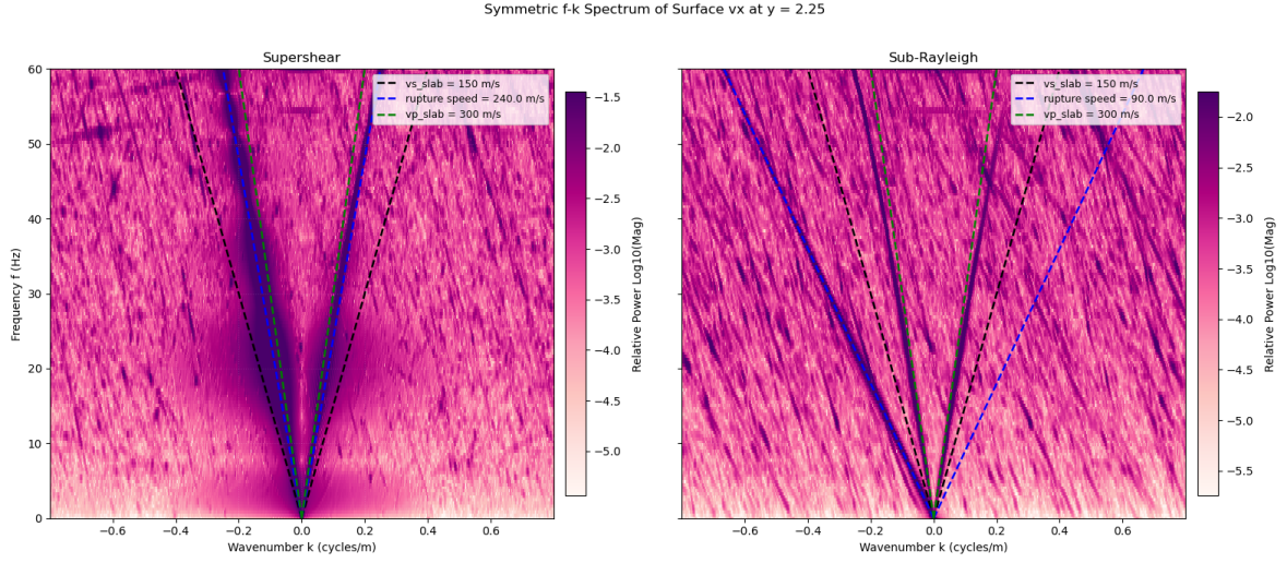
Figure 4.3: F-k plot for the supershear (left) and sub-rayleigh (right) case. Slab p-wave velocity in green, s-wave velocity in black and respective rupture speed in blue. Colorbar shows relative energy (log10 of the magnitude of energy).
