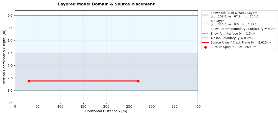
Figure 3.1: Layered model setup. Air layer in light blue, snow layer in darker blue. Source line extent in red.
