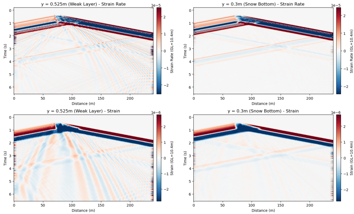
Figure 4.8: Strain and strain rate (horizontal component) averaged over 10.4m gauge length to represent DAS data: strain rate in top column, strain in bottom column. Crack depth on left, snow bottom on the right. Colorbar shows magnitude of strain or strain rate.
