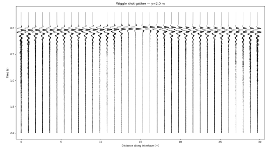
(b) Wiggle plot for moment tensor source.
