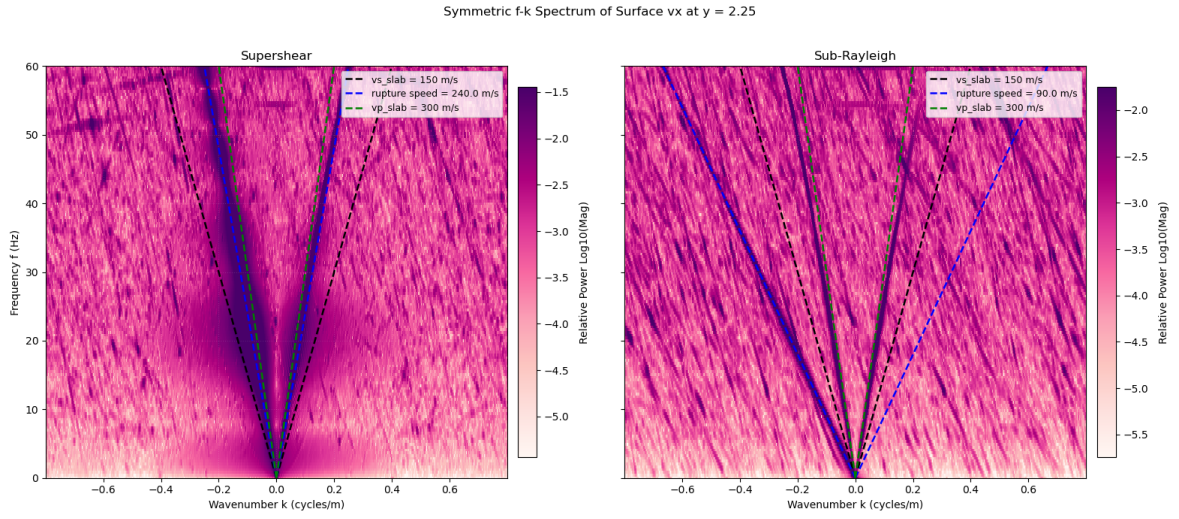
Figure 4.3: F-k plot for the supershear (left) and sub-rayleigh (right) case. Slab p-wave velocity in green, s-wave velocity in black and respective rupture speed in blue. Colorbar shows relative energy (log10 of the magnitude of energy).
