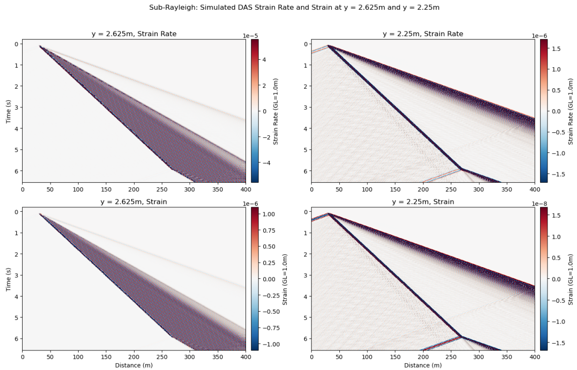
Figure H.1: Sub-Rayleigh strain and strain rate (horizontal component) averaged over 1 m gauge length to represent DAS data: strain rate in top column, strain in bottom column. Crack depth on left side, snow bottom on right side. Colorbar shows magnitude of strain or strain rate, colorbars unscaled.
