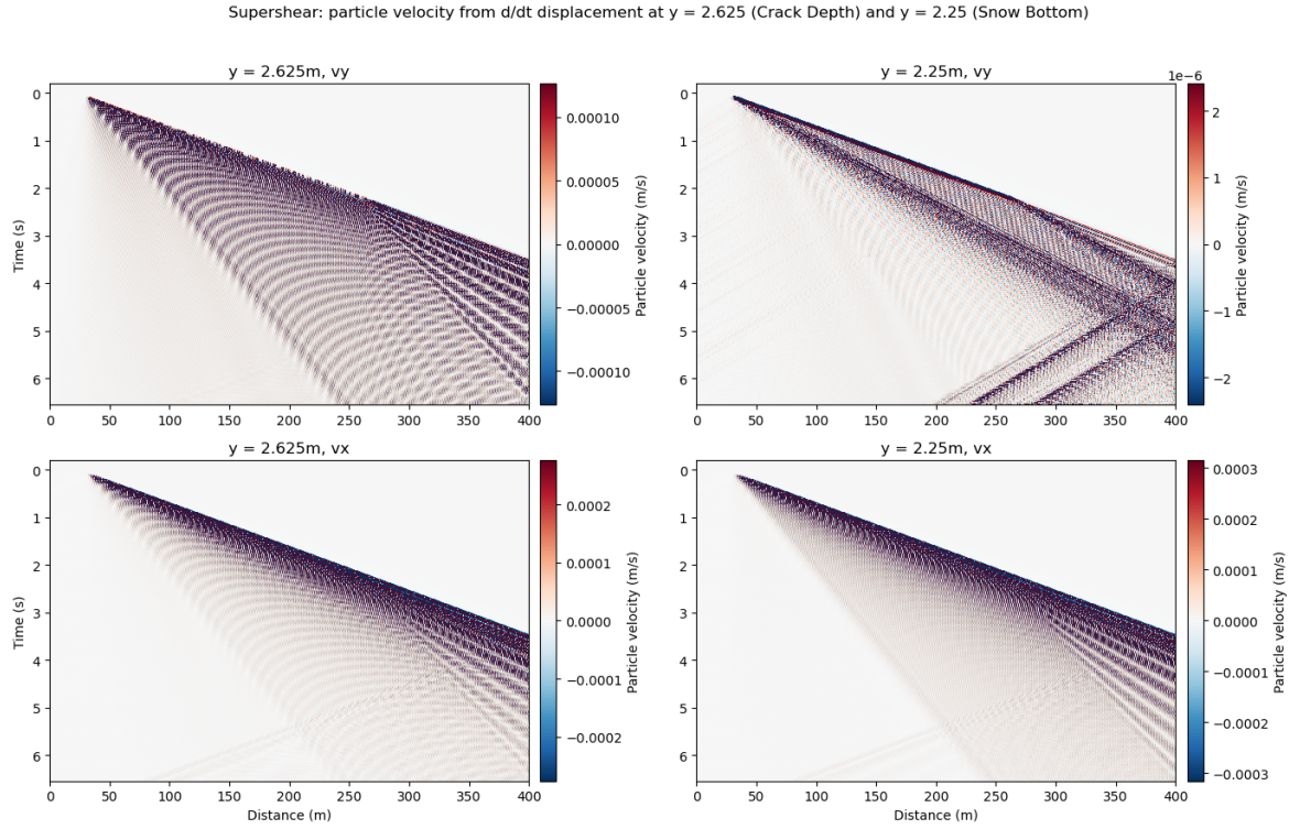
Figure 4.7: CZM Supershear Particle velocity: vertical velocity in top row, horizontal in bottom row. Crack depth in left, snow bottom in right column. Colorbar is unscaled, showing velocity (m/s).
