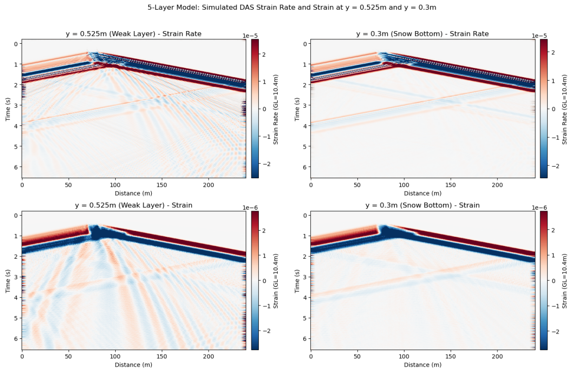
Figure 4.8: Strain and strain rate (horizontal component) averaged over 10.4m gauge length to represent DAS data: strain rate in top column, strain in bottom column. Crack depth on left, snow bottom on the right. Colorbar shows magnitude of strain or strain rate.
