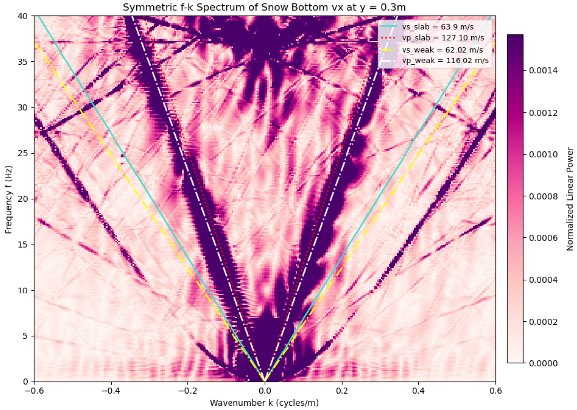
Figure 4.11: F-k plot for the MPM-guided simulation. Slab P-wave velocity in red, slab S-wave velocity in turquoise. Weak layer P-wave velocity shown by the white layer, S-wave velocity of WL shown by yellow line. Colorbar shows energy normalized to the 99th percentile to avoid outliers.
