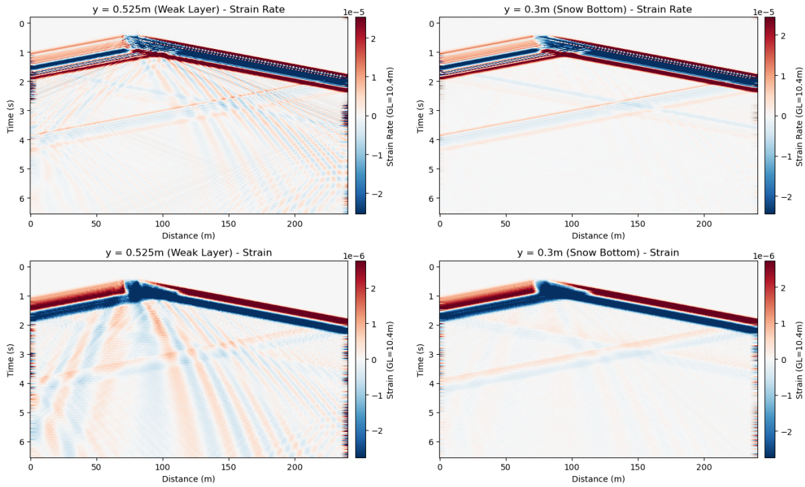
Figure 4.8: Strain and strain rate (horizontal component) averaged over 10.4m gauge length to represent DAS data: strain rate in top coulumn, strain in bottom column. Crack depth on left, snow bottom on the right. Colorbar shows magnitude of strain or strain rate.
