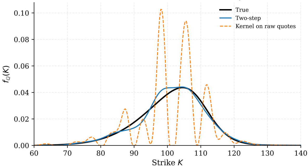
Heston draw where the raw kernel misses by the most
