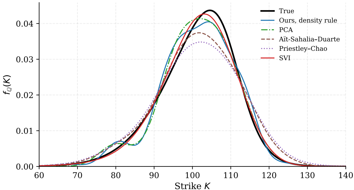
Heston, one draw at the median density-rule ISE
