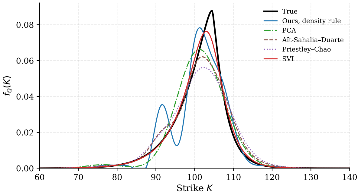
Variance gamma, one draw at the median density-rule ISE
