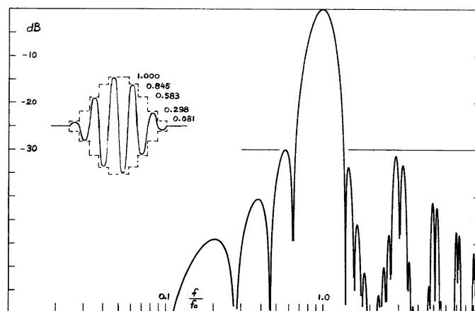
Fig. 8. Spectrum of a five-cycle tone burst which is assembled from half sine waves of different amplitudes to approximate a raised-cosine envelope. The discrete slope changes at zero crossings produce odd-order harmonics. The spectral content compares favorably with the exact raised-cosine envelope spectrum and is an improvement over the rectangular envelope (Figs. 1 and 3).
